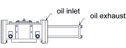
Double Acting Hydraulic Actuator
